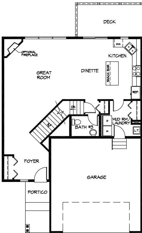
MAIN FLOOR 952 SQ. FT.
